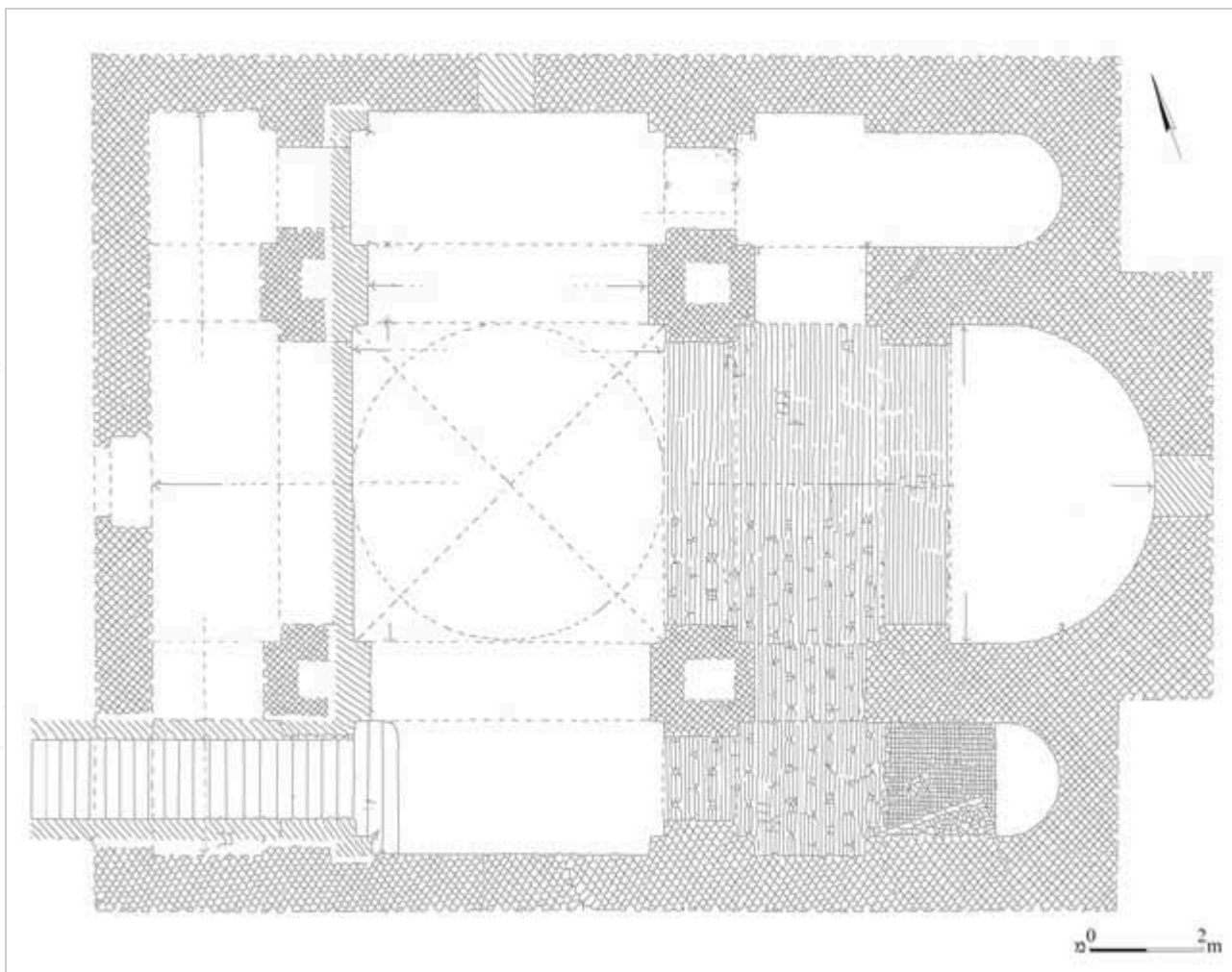
圖 2：Plan of the ancient church according to Vincent and Abel (1922:599).
