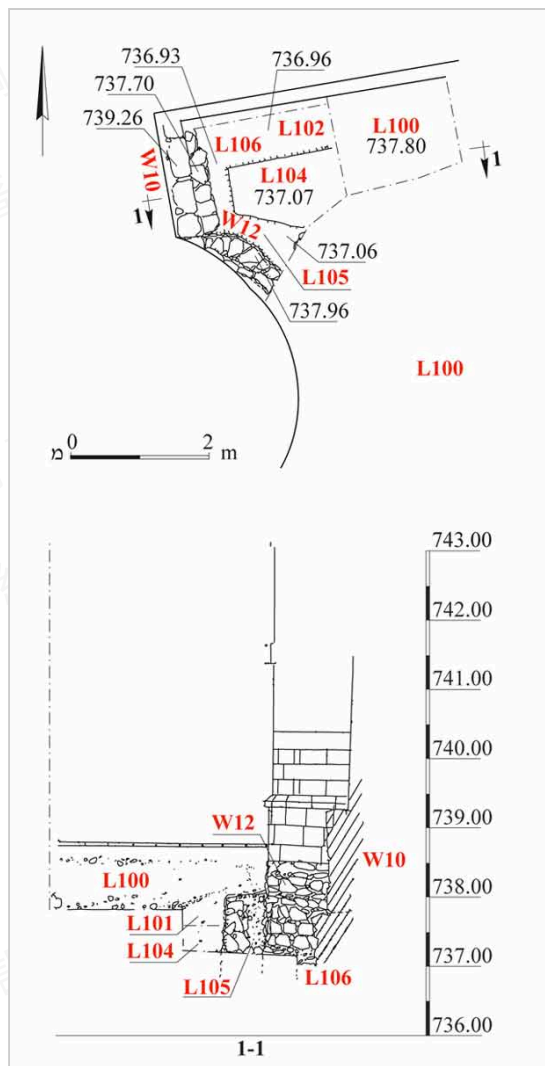
圖 3 : The excavation area, plan and section.
