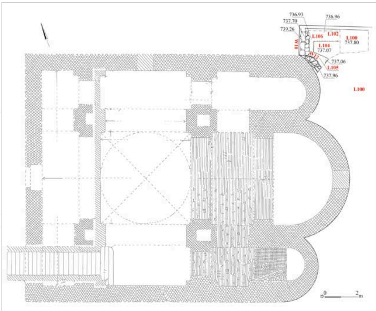
圖 6：The excavation plan and the front of the apse integrated in a corrected plan of Vincent and Abel (see Fig. 2).
